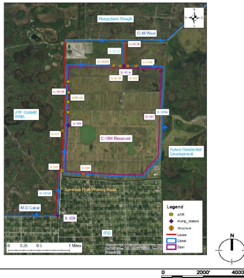
C-18W IMPOUNDMENT STRUCTURES AND FLOWS
