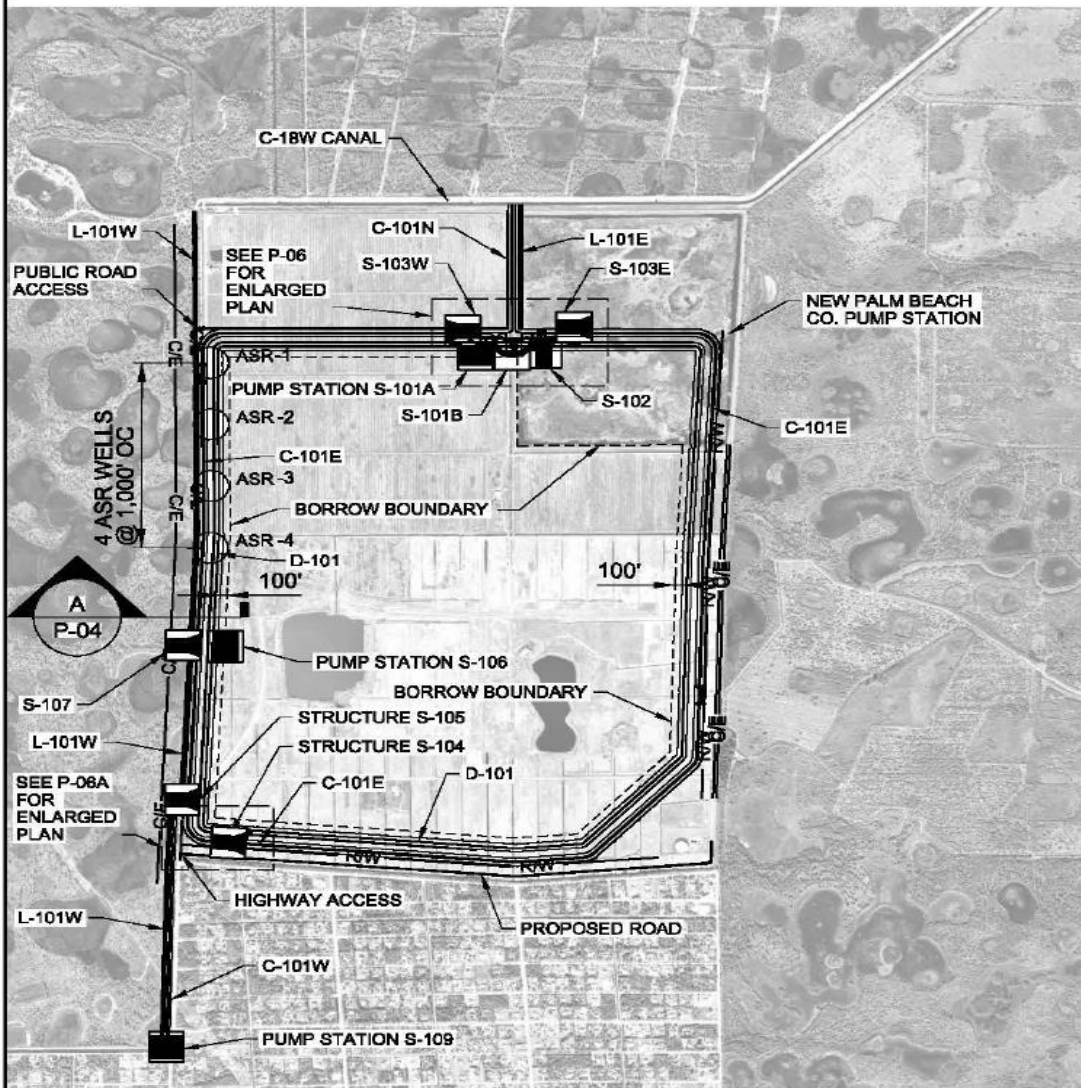
C-18W IMPOUNDMENT SITE PLAN
